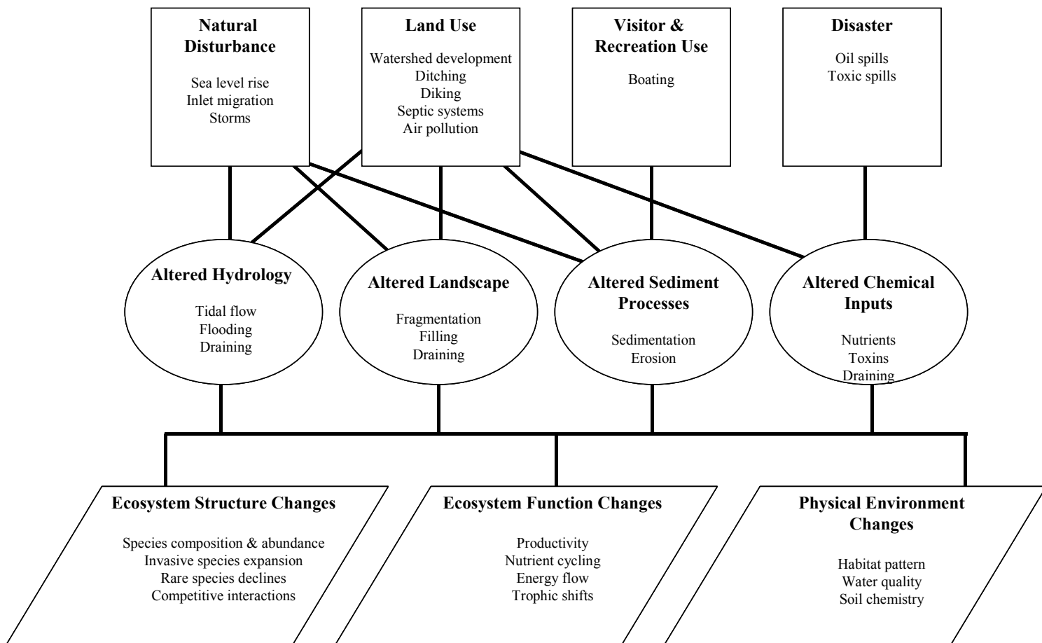
Figure 2.2 Northeast Coastal and Barrier Network Salt Marsh Ecosystem Model
